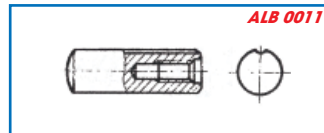
Dowel Pin with Internal Thread
