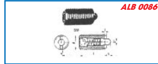
Spring Plunger
